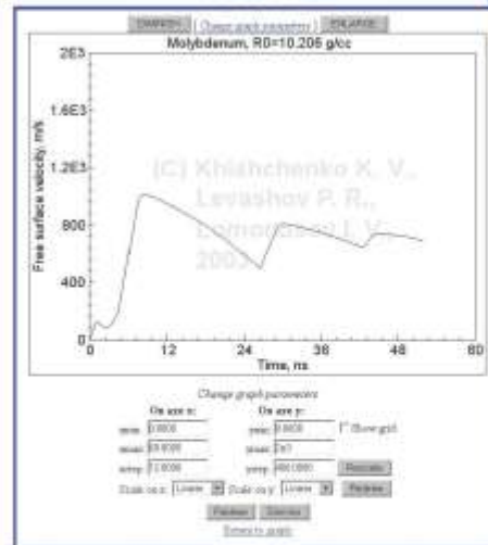
Free surface velocity profile Sample: Mo, 0.416 mm thick Striker: Al, 0.05 mm thick, velocity 4100 km/c
