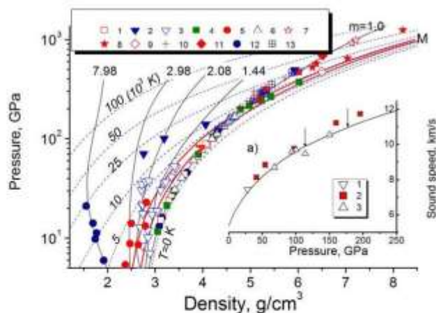
Fig. 9. Phase diagram of aluminum at high pressures. Nomenclature: lines—EOS calculations, T—isothers, M—melting region, m —shock adiabat of porous samples ( m = \rho_0/\rho_{00} —porosity); points—experimental data, 1—Al'tshuler et al. (1981), 2—Kormer et al. (1962), 3—van Thiel (1977); 4—Al'tshuler et al. (1960a); Al'tshuler & Chekin (1984), 5—Bakanova et al. (1974), 6—Mitchell & Nellis (1981), 7—Simonenko et al. (1985), 8—revision Trunin et al. (2001) of original data Avrorin et al. (1987), 9—Trunin (1986), 10—Glushak et al. (1989), 11—Trunin et al. (1995a), 12—Trunin et al. (2001), 13—Knudson et al. (2003). a) Sound speed in shocked aluminum. Line—EOS, points—experiment, 1—Neal (1975), 2—Al'tshuler et al. (1960b), 3—McQueen et al. (1984), arrows indicate the melting region.
