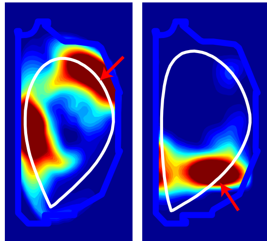
Figure 1. Cooling Superhot Plasma - Comparison of experimentally measured radiated power emission patterns inside the DIII-D tokamak with upper gas injection (left) and lower gas injection (right). Arrows indicates gas valve locations, the white border represents the plasma boundary, and the light blue border shows the vacuum vessel. Red coloring indicates the strongest emission, blue weakest.
