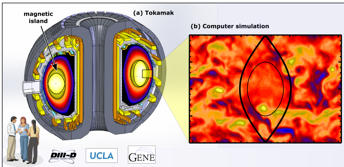
Figure 1. (a) Schematic view of the DIII-D tokamak showing magnetic islands, (b) computer simulations of a magnetic island and turbulence.
