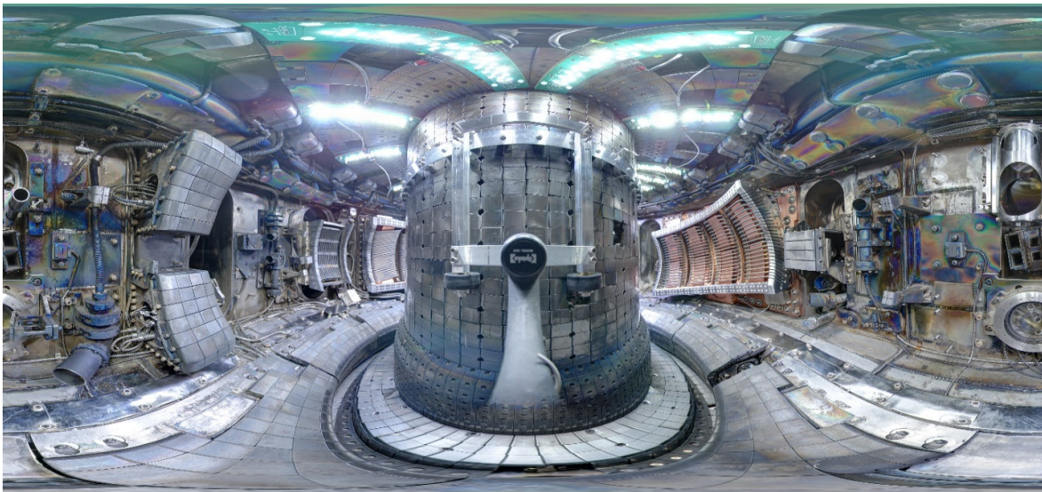
Figure 1. A fish-eye view of the interior of the C-Mod tokamak experiment. A 3D video tour of the C-Mod facility can be found at https://www.youtube.com/watch?v=nkMM61e8Ajw
