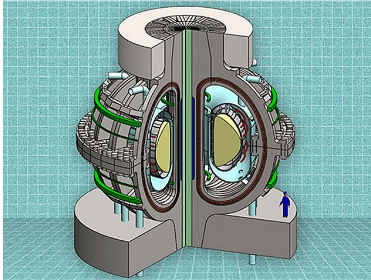
Figure 1: Conceptual design of the ARC fusion reactor. About the same size as the currently operating JET tokamak in the United Kingdom, but with three times the magnetic field strength, ARC is sized to produce 500 MW of deuterium-tritium fueled fusion power.
