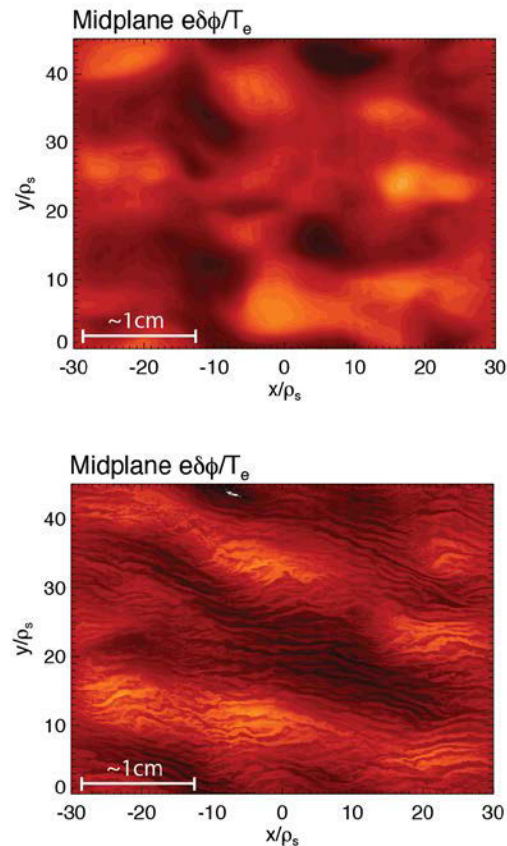
Figure 1: Plasma turbulence in conditions with long wavelength turbulence (top) are compared with those exhibiting long and short wavelength turbulence (bottom). The top condition is representative of the standard model. The bottom model demonstrates the clear impact of capturing long and short wavelength turbulence simultaneously.
