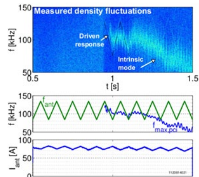
Figure 1: (Top) Time-resolved power spectrum of density fluctuations driven by the Shoelace Antenna. The driven fluctuations begin a little before 1 second (marked by the triangular feature) and follow a driven response to the antenna. Later at around 1.25 seconds the intrinsic plasma fluctuations become the dominant feature in the spectrum. (Middle) Frequency of antenna drive and peak frequency of the intrinsic density fluctuation. (Bottom) Electrical current amplitude flowing in the shoelace winding of the antenna.
