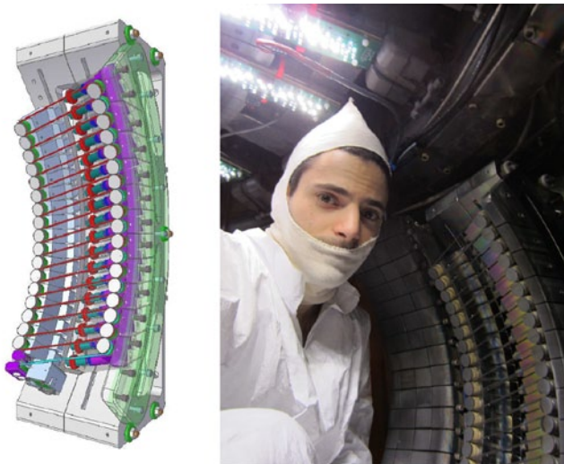
Figure 2: (Left) CAD model of antenna (Image: R. Leccacorvi). The Shoelace Antenna - a novel structure developed at MIT's Alcator C-Mod tokamak to drive short-wavelength fluctuations at the plasma boundary. The antenna gets its name from the crisscross pattern traversed by its single winding of molybdenum-wire, shown in red in the model. Electrical current flows at radio frequencies through the crisscrossing wire pattern to induce fluctuations in the plasma. (Right) Antenna mounted inside the Alcator C-Mod vacuum vessel. One of the authors sits alongside, wearing special clothing to keep the machine interior clean (Photo: T. Golfinopoulos).
