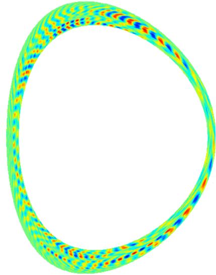
Figure 1. Cross-section of annular region showing edge pedestal turbulence due to instabilities found using first-principle, five-dimensional kinetic simulations.
