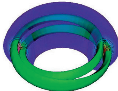
Figure 1. Computer simulation showing the structure of a magnetic island (green) in the toroidal geometry of the DIII-D tokamak, and the hot fusion core (red). [Figure provided with permission from D.P. Brennan, “Modeling with the NIMROD code.”]
