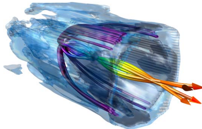
Example of a laser wakefield simulated in a “Boosted Frame”. Electrons (colored tubes) are injected and accelerated by surfing the wave (blue surfaces) generated by a laser pulse.
